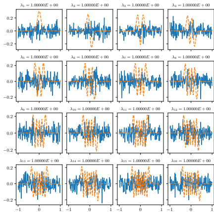
(a) 16 first eigenvectors obtained with an eigendecomposition (solid blue curve) of \mathbf{K}(0) , compared to the exact eigenvectors (dashed orange curve). Here, \widehat{m}_F = \mathbf{1}_{[-0.49 \cdot 2\pi\mu(\varepsilon), 0.49 \cdot 2\pi\mu(\varepsilon)]} . N_1 = 150, \eta = 10^{-10} .
