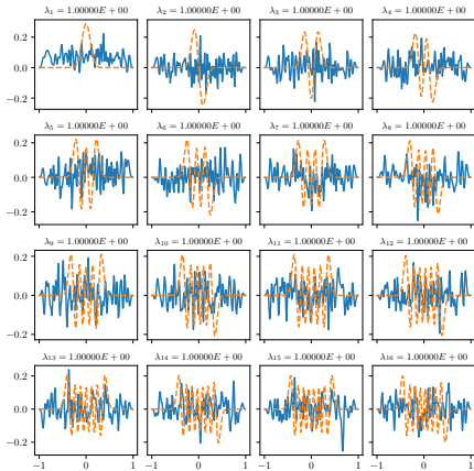
(a) 16 first eigenvectors obtained with an eigendecomposition (solid blue curve) of \mathbf{K}(0) , compared to the exact eigenvectors (dashed orange curve). Here, \widehat{m}_F = \mathbf{1}_{[-0.3 \cdot 2\pi\mu(\varepsilon), 0.3 \cdot 2\pi\mu(\varepsilon)]} . N_1 = 150, \eta = 10^{-10} .
