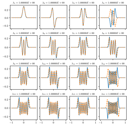
(b) 16 first eigenvectors obtained with the varying masks procedure (solid blue curve) of \mathbf{K}(0) , compared to the exact eigenvectors (dashed orange curve). Here, \widehat{m}_F = \mathbf{1}_{[-0.3 \cdot 2\pi\mu(\varepsilon), 0.3 \cdot 2\pi\mu(\varepsilon)]} . N_1 = 150, \eta = 10^{-10} .
